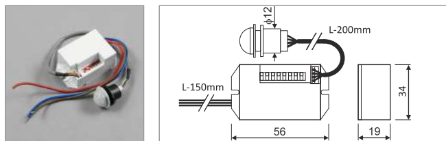
movement sensor YCB1050 czujnik ruchu YCB1050 230V/800W
